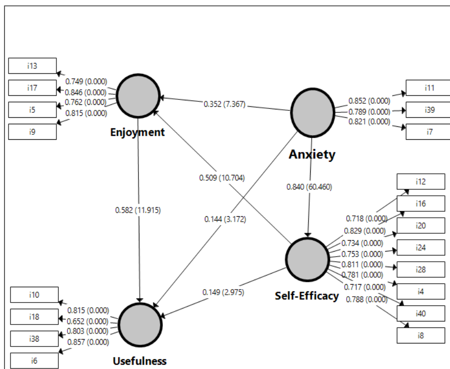
Figure 2 IAS Structural Model results for Spain and Romania (complete population)
