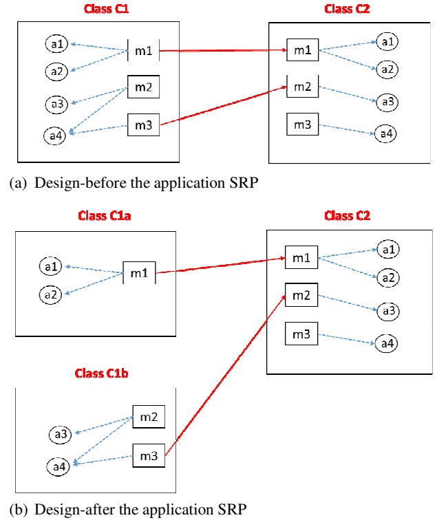
Figure 1. Modularity Example
