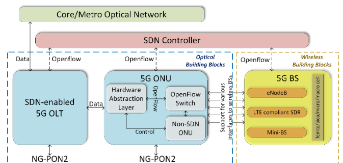
Fig. 3. 5G hybrid optical-wireless ONU
