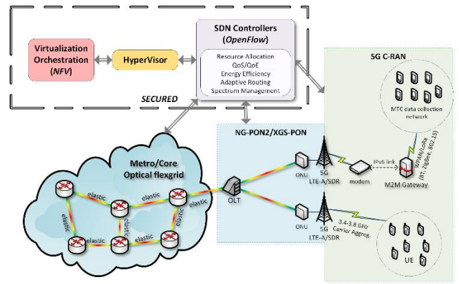
Fig. 2. Overview of the proposed architecture
